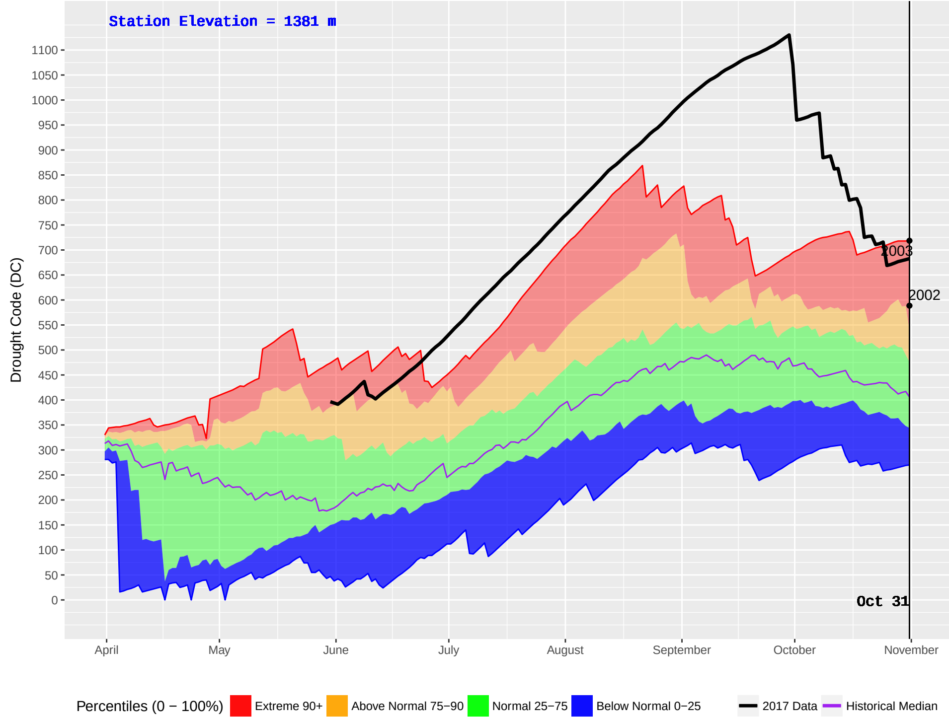
GLIMPSE (291) : Historical (1978–2016) and Current (2017) Noon Drought Code (DC)
