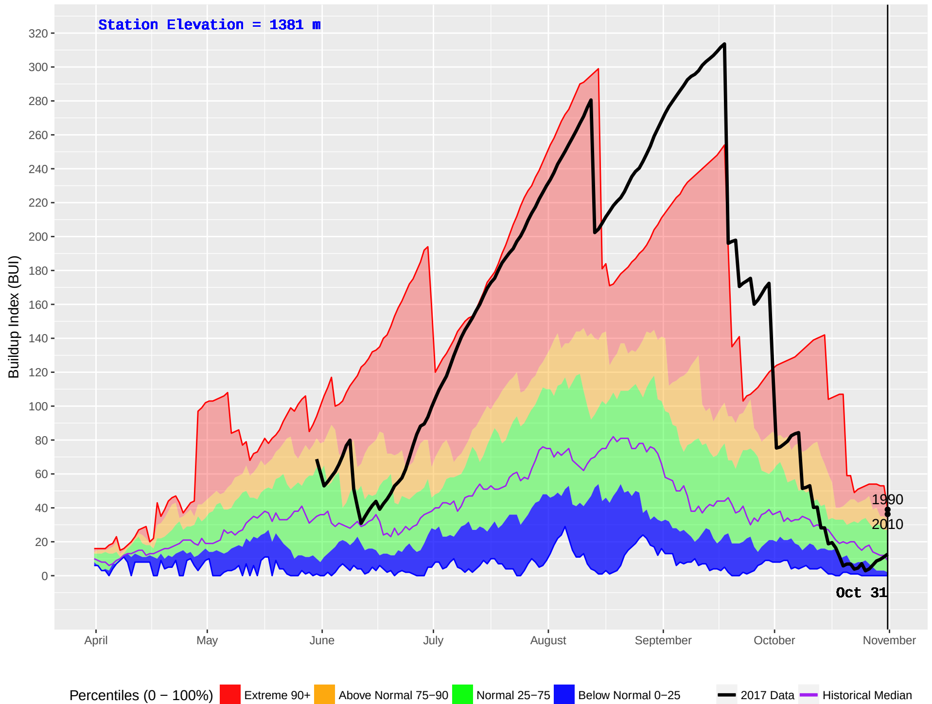
GLIMPSE (291) : Historical (1978–2016) and Current (2017) Noon Buildup Index (BUI)
